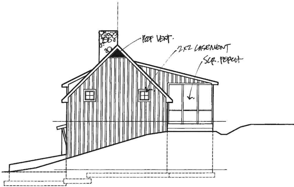
SOUTH ELEVATION \frac{1}{8}'' = 1'-0''
