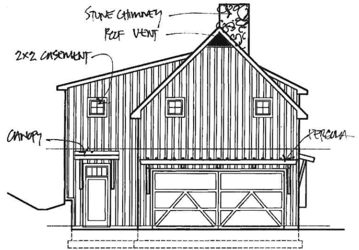
NORTH ELEVATION \frac{1}{8}'' = 1'-0''
